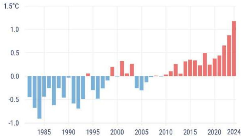
Figure 3.2. Trends in SST anomalies across the Mediterranean. Source: Fig 11.1 of ESOTC, 2024.
